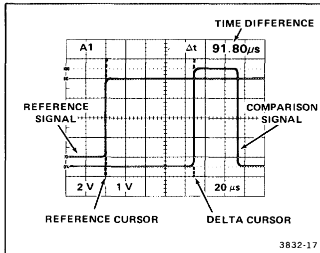
Figure 6-5. Time difference between two time-related pulses (cursor method).
