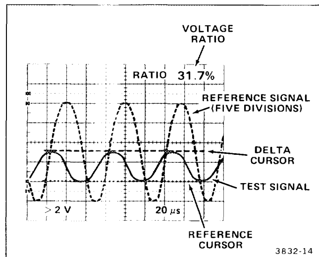
Figure 6-2. Voltage ratios.
